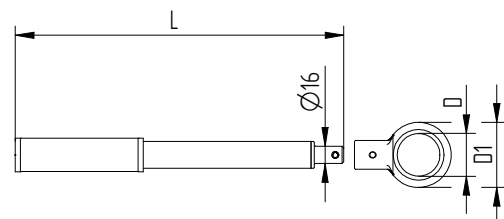
G-A/G-AS with A-FLS
