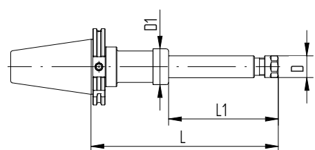
SK/ER XL (form A+AD)
